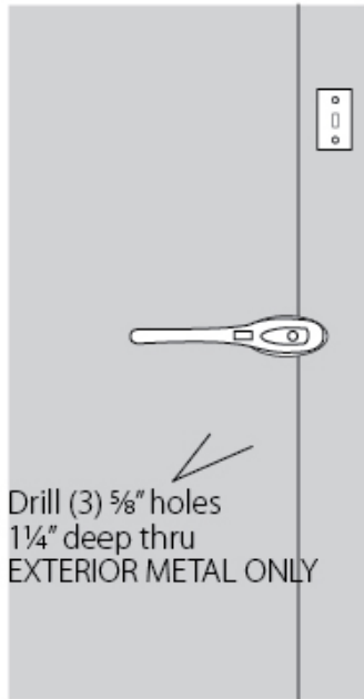
FIGURE 7 Door Exterior
