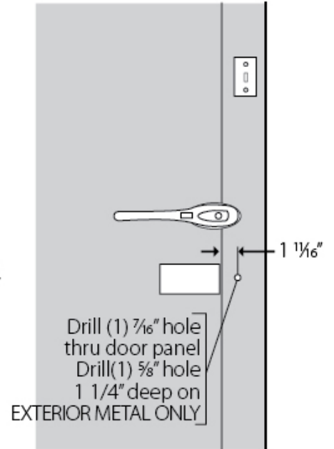
FIGURE 9 Door Exterior
