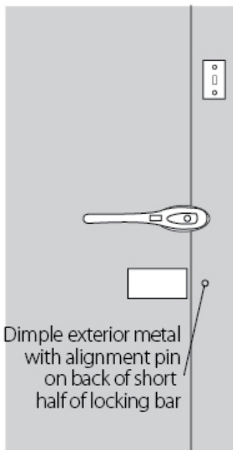
FIGURE 10 Door Exterior
