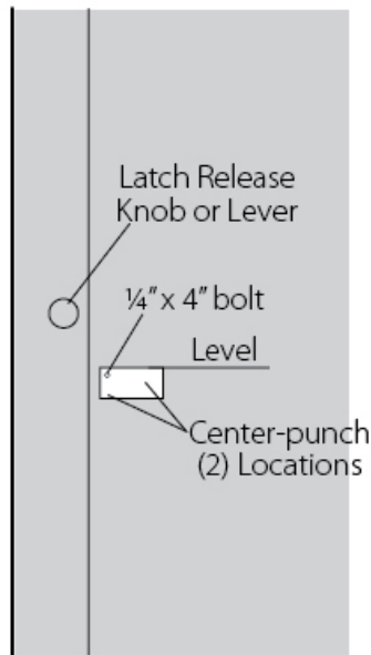
FIGURE 5 Door Interior
