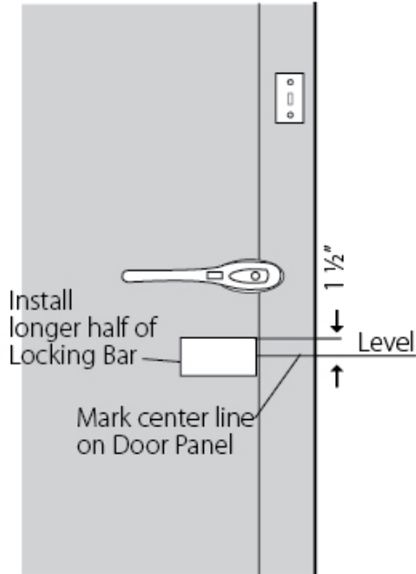
FIGURE 8 Door Exterior
