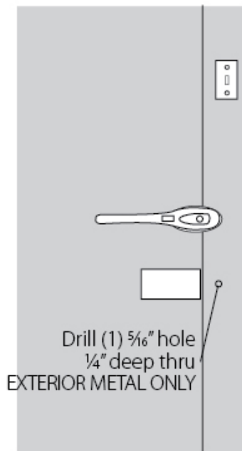
FIGURE 11 Door Exterior
