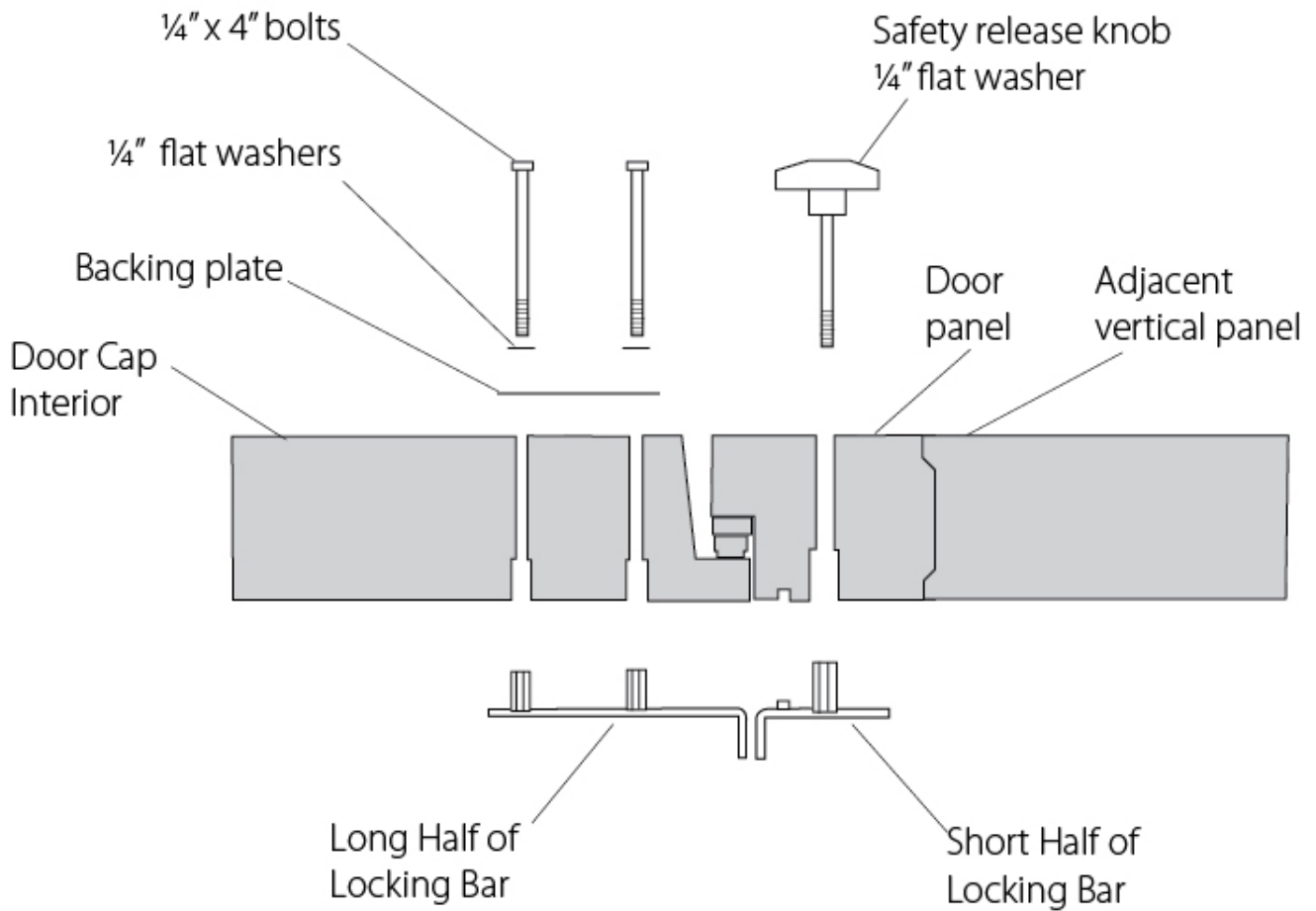
Exploded view of assembly section of door latch side
