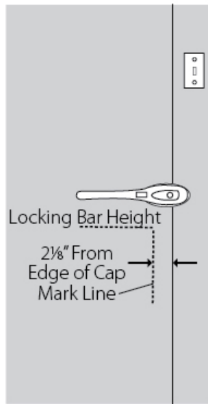
FIGURE 2 Door Exterior
