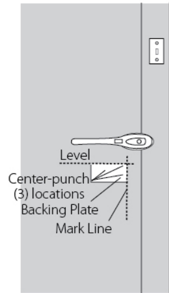
FIGURE 3 Door Exterior
